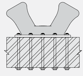
Steelwork Mounting Type
