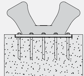
Retrofit Mounting Type (using EC 2 epoxy anchors)
